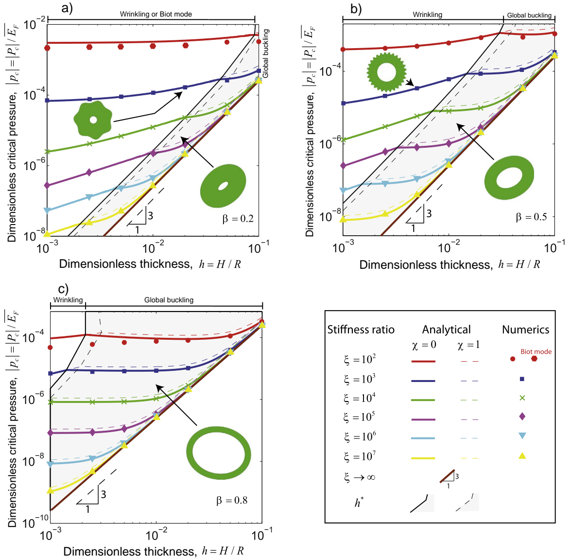
Fig. 4. Dimensionless critical pressure |p_c| = |P_c|/E_F versus the dimensionless ring thickness h = H/R , for several stiffness ratios \xi = E_F/E_S and cavity sizes \beta : (a) \beta = 0.2 , (b) \beta = 0.5 and (c) \beta = 0.8 . Theory (lines) is given by Eq. (17). Poisson's ratio of the substrate is \nu_S = 0.5 . The legend (bottom right) is common to all three plots.
