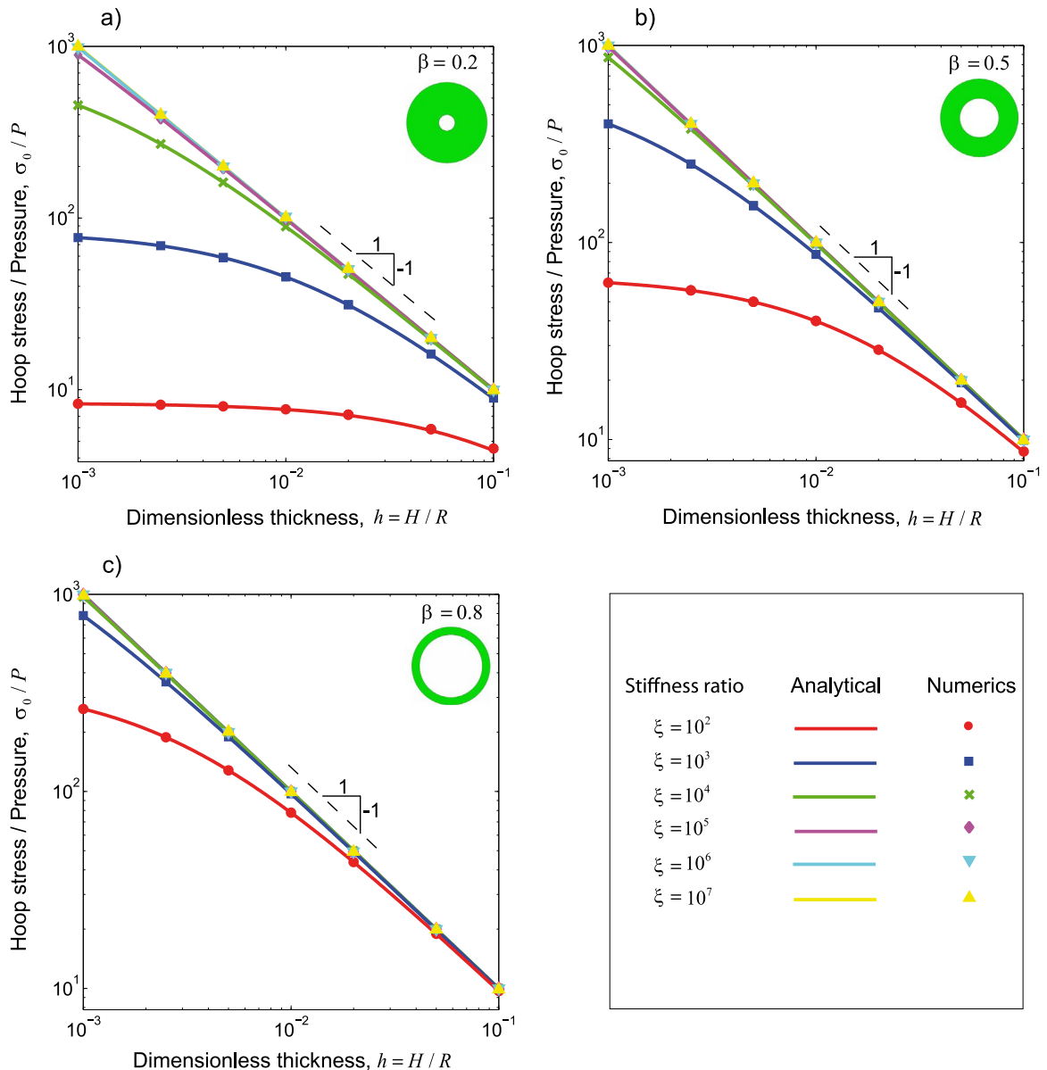
Fig. 3. Pre-instability hoop stress, \sigma_0 , in the ring, normalized by the pressure, P , as a function of the dimensionless ring thickness, h = H/R . Cavity sizes are (a) \beta = 0.2 , (b) \beta = 0.5 and (c) \beta = 0.8 . Poisson's ratio of the substrate is \nu_S = 0.5 . Analytical predictions are given by Eq. (12) as solid lines and FEM results are plotted as data points. The legend (bottom right) is common to all three plots.
