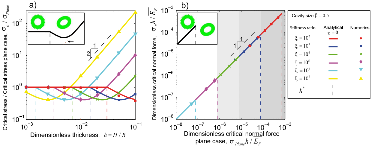
Fig. 6. (a) Critical stress \sigma_c normalized by its planar substrate counterpart, \sigma_{plane} , as a function of the dimensionless ring thickness h = H/R . (b) Dimensionless critical normal force versus planar substrate counterpart. Analytical predictions (solid lines) are given by Eq. (21a) and FEM results are shown as data points. Insets are sketches of the wrinkling and global buckling modes. The cavity size is \beta = 0.5 and the Poisson's ratio of the substrate is \nu_s = 0.5 . The legend is common to both plots.
