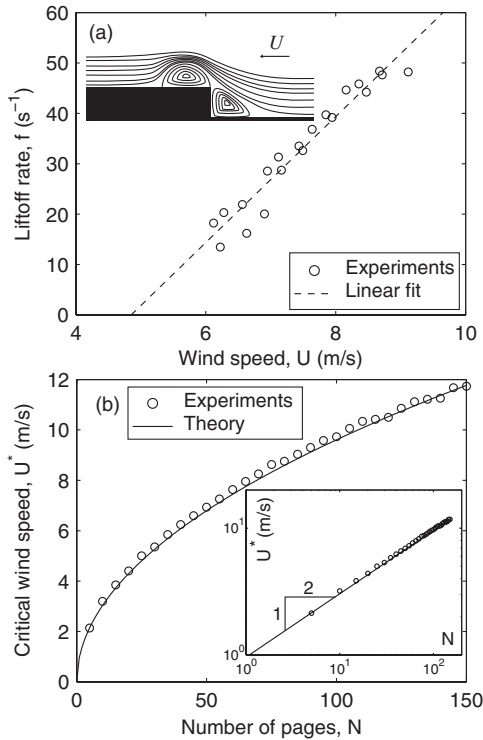
FIG. 3. (a) Experimental page liftoff rate for the paper book. The dashed line is the liftoff rate given by Eq. (5). Inset: Sketch of expected flow profile. (b) Critical wind speed measured for an elevated stack of N pages. The solid line is calculated using Eq. (6). Inset: log-log version of the plot.
