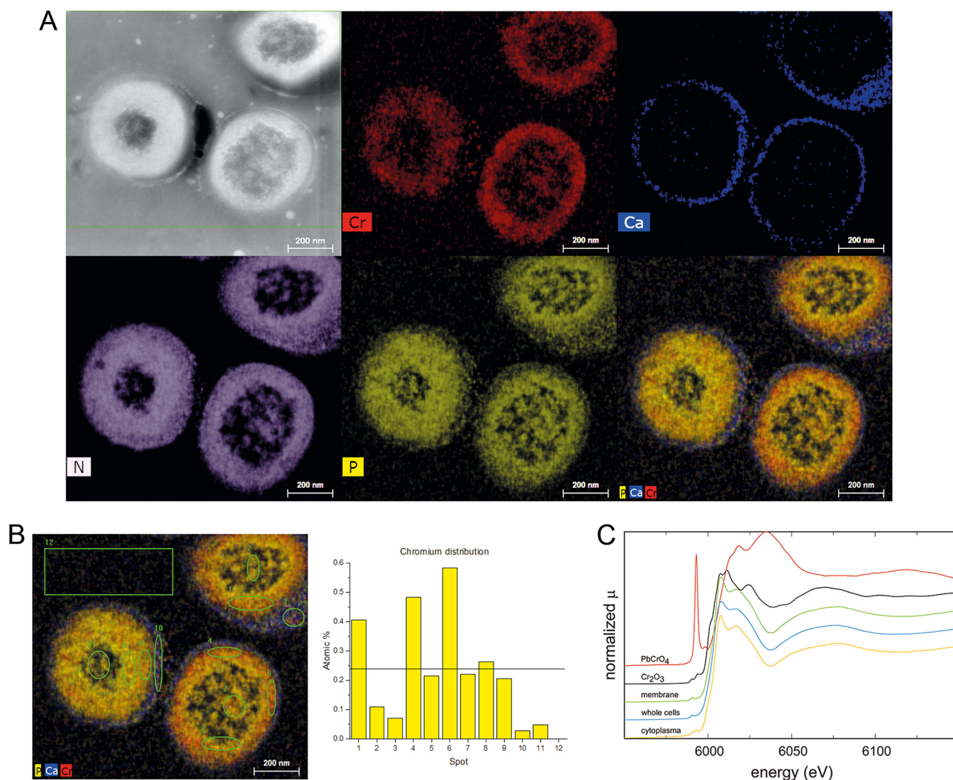
FIG 4 Chromium distribution in L. chromiirestiens extracellular matrix. (A) EDS images of chromate-grown cells. STEM overview (HAADF) and element distribution. Cr, chromium; Ca, calcium; N, nitrogen; P, phosphorus; PCaCr, superimposition of P, Ca, and Cr signals. (B) Detailed element analysis of the chromium dispersion. The spots are indicated on the left, and the corresponding atomic percentages of chromium are shown on the right. The black line indicates the mean chromium content of all analyzed spots (1 to 11). (C) Determination of chromium oxidation status via XANES. The predominant chromium species bound to cells was identified as \text{Cr}^{3+} .
