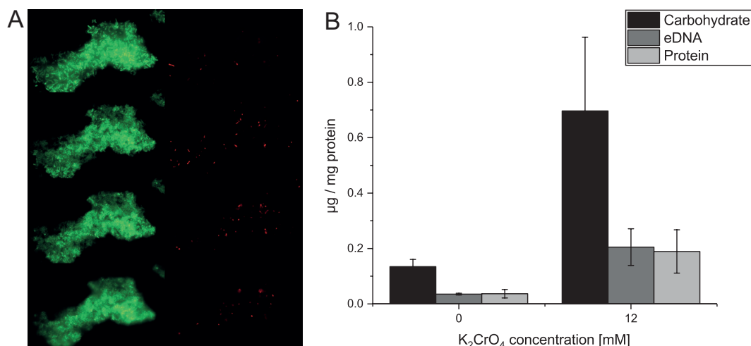
FIG 2 Chromate stress-induced aggregate formation of L. chromiirestiens . (A) LIVE/DEAD stain of a representative aggregate. Green, 4',6-diamidino-2-phenylindole (DAPI) stain (all cells); red, propidium iodide stain (cells with collapsed membrane potential). Shown are 4 different Z-levels of the aggregate. (B) EPS components of cellular aggregates of L. chromiirestiens cells grown without (0 mM) and with (12 mM) K 2 CrO 4 . The quantity of each of the tested components increased as a response to growth under chromate stress. All values were normalized to the initial amount of biomass (quantified as total cell protein) that was used for EPS isolation. Error bars represent SD of the results from three independent replicates.
