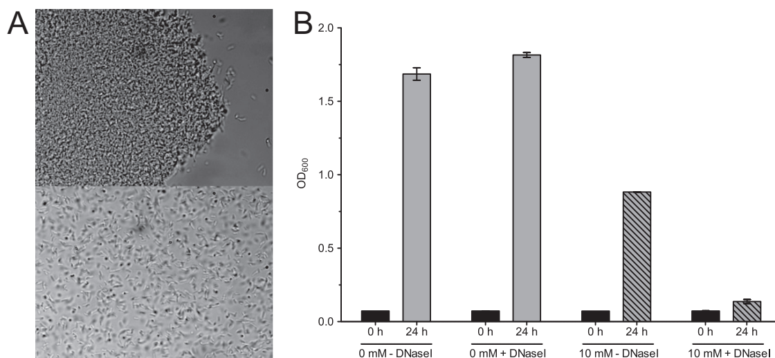
FIG 3 Key role of eDNA. (A) Phase-contrast micrograph ( \times 1,000 ) prior to (top) and 10 min after (bottom) the addition of DNase I. The addition of DNase I leads to a rapid disintegration of cellular aggregates. (B) Growth of L. chromiiresistens in the presence and absence of DNase I. The graph shows the OD values at the start of the experiment (0 h) and after 24 h. The addition of DNase I (+DNase I) did not affect the final OD achieved without chromate supplementation, while it severely impacted growth in the presence of 10 mM chromate. Error bars represent SD of the results from three independent replicates.
