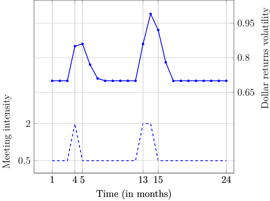
Figure 9: Volatility Clustering.
