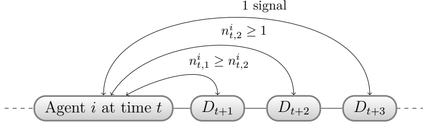
Figure 2: Information Percolation.
