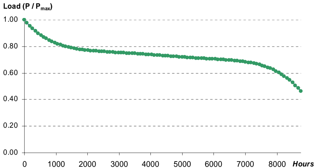
Figure 12. Normalised Load Duration Curve of Western Europe Region in 2000
