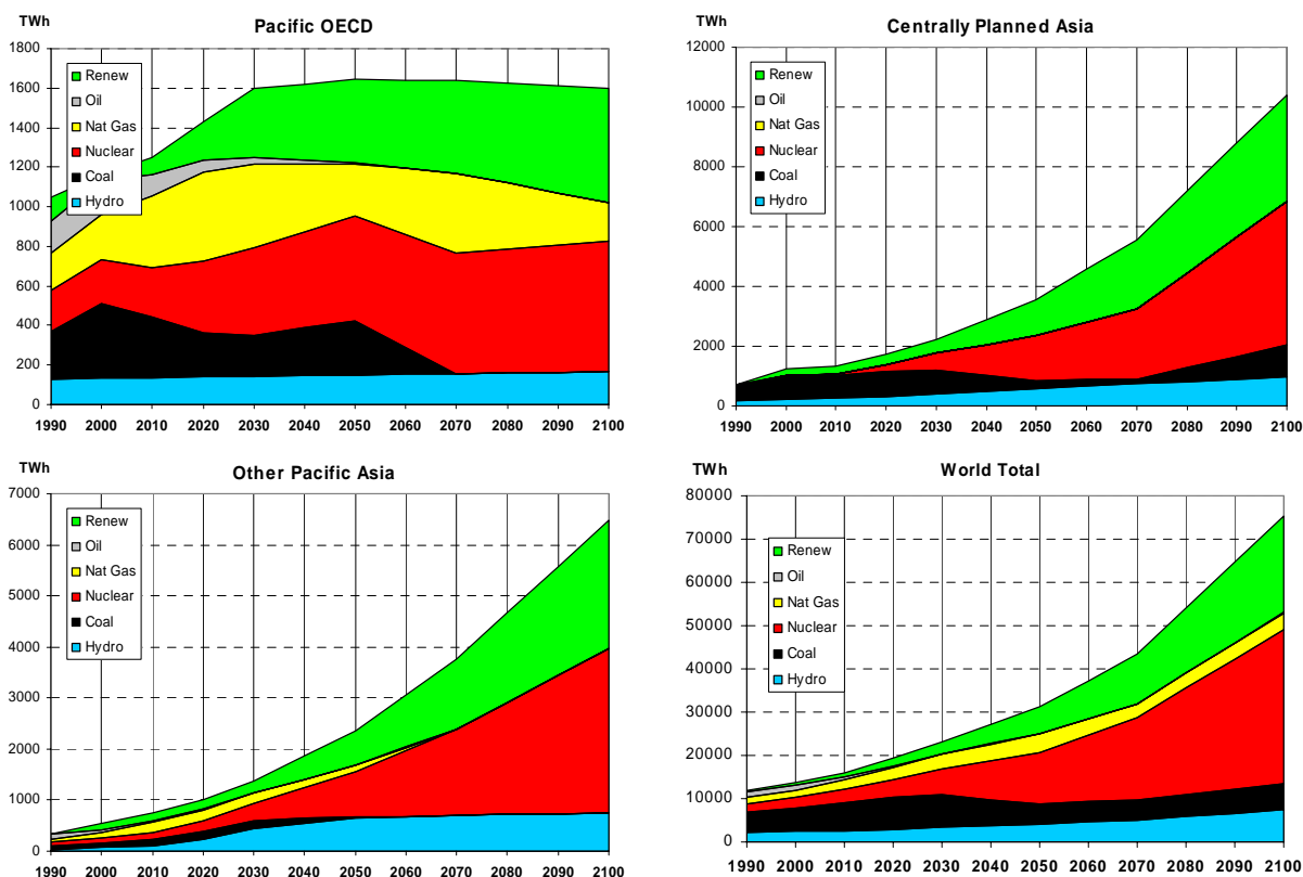
Figure 8-b. Electricity Generation Structure by Fuel Type in IASA / WEC – Scenario “B”
