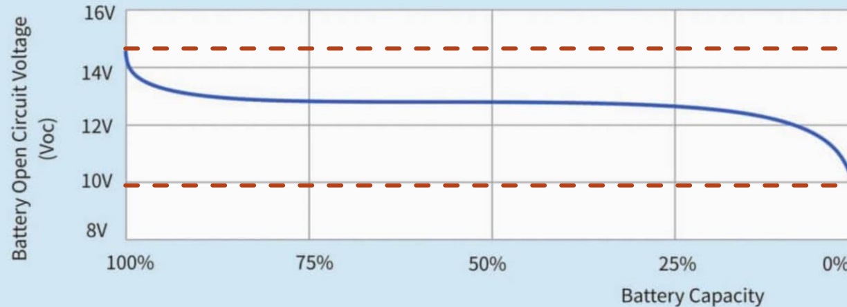
12V LiFePO4 Battery Voltage Chart
